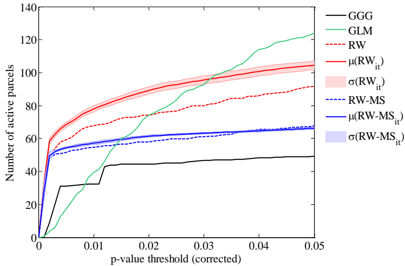
Fig. 2. Quantitative activation detection comparison.
